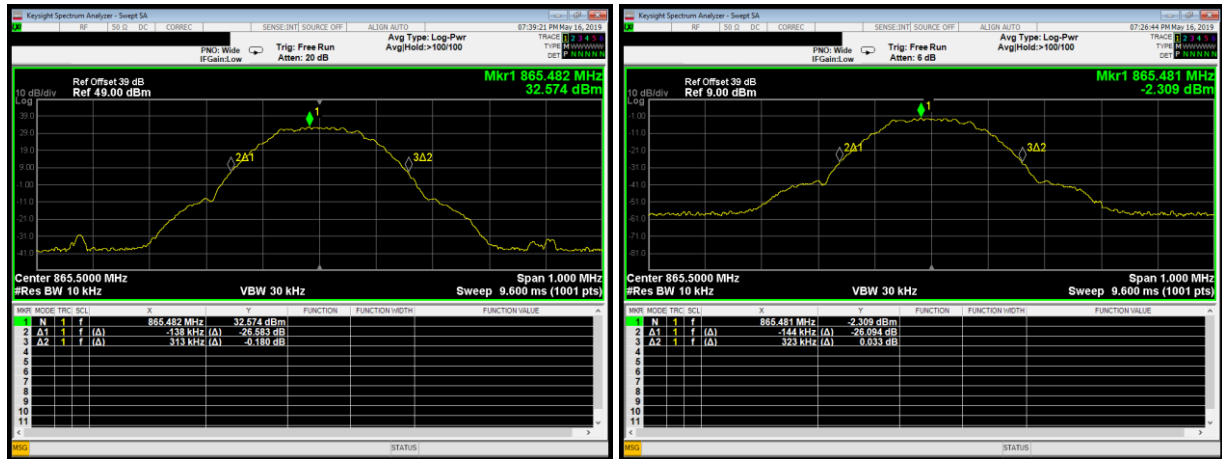
Plot 3.2.1: Input-versus-output signal comparison, MSK, Gaussian filter 0.3, data rate 270kbps, 0.5 dB below AGC threshold level
