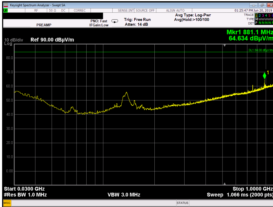
Plot 3.6.5: Spurious Emissions test results, 30 MHz – 1 GHz range, Horizontal polarization, Middle Frequency
