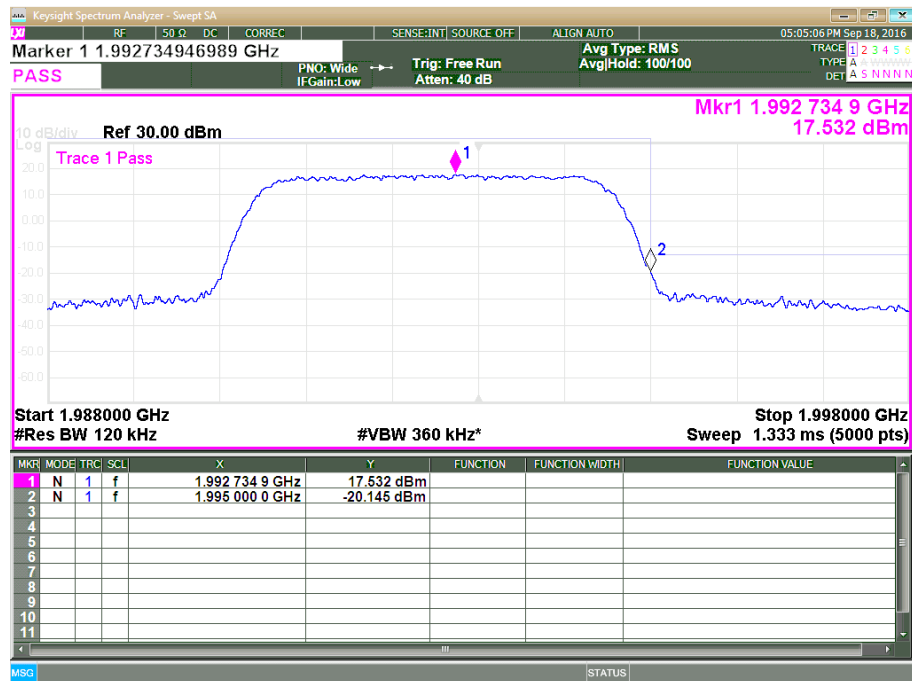
Plot 3.4.7: Band Edge test results, AWGN 4.1MHz, F_c = 1992.50 MHz, single test signal
