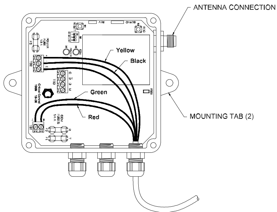
Figure 1: Line Module Wiring
