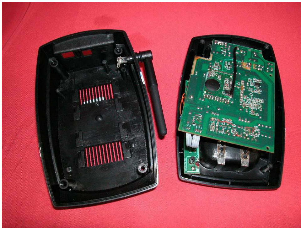
Base assembly (View 2)
