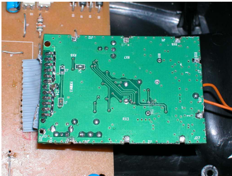
Base Oscillator PCB solder side
