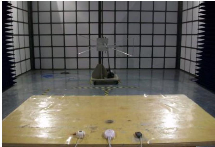
Radiation Emission Test View For 30MHz-1000MHz
