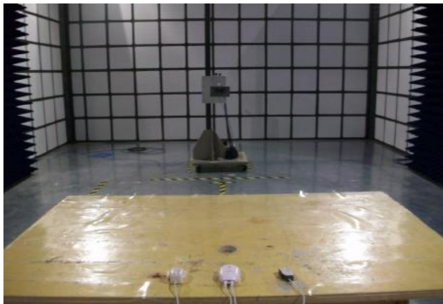
Radiation Emission Test View For 1GHz-5GHz
