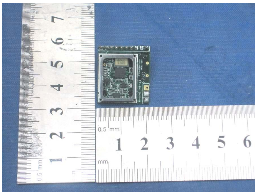
2.8EUT-PCB4 - Back View
