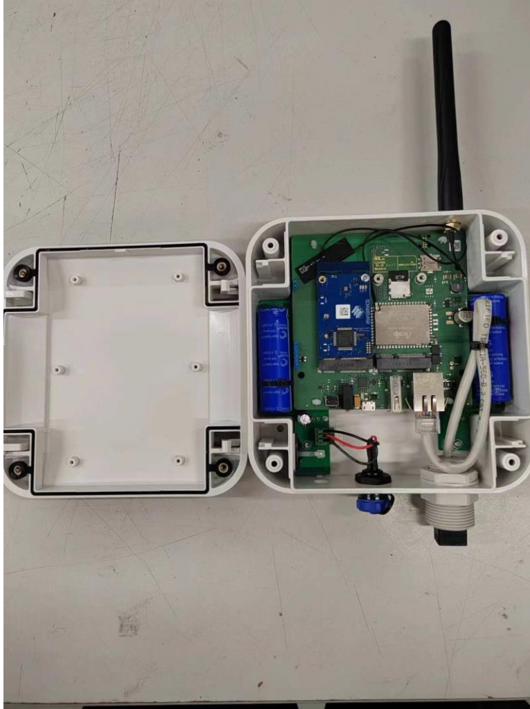
Main board
