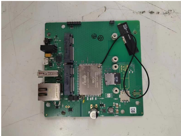
Main board
