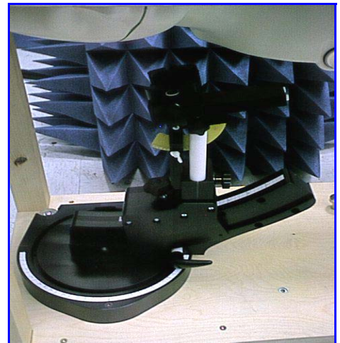
Figure 5. Device Holder
