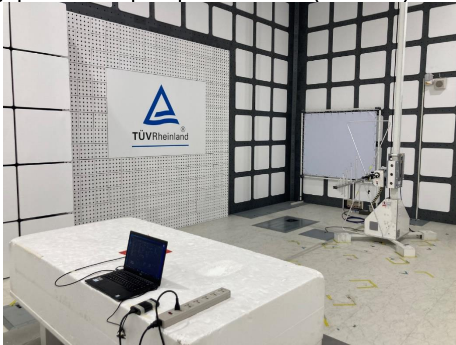
Photograph 11: Test Setup for Spurious Emissions (Back View 2)
