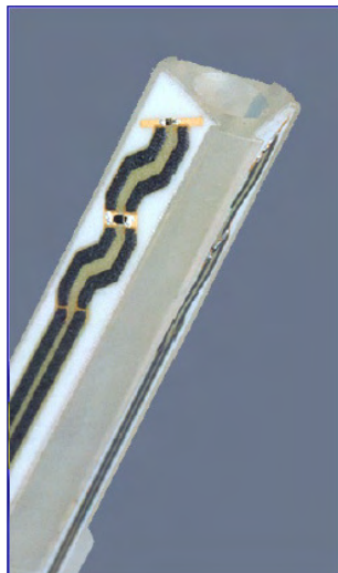
Figure 3. E-field Probe
