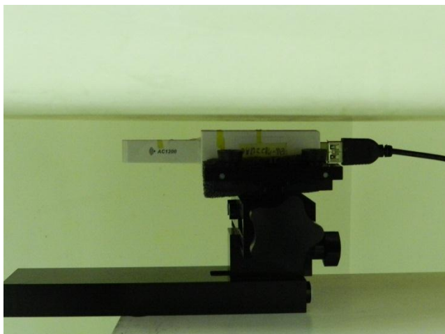
Vertical Back with Phantom 5 mm Gap Antenna swivel 180 degree
