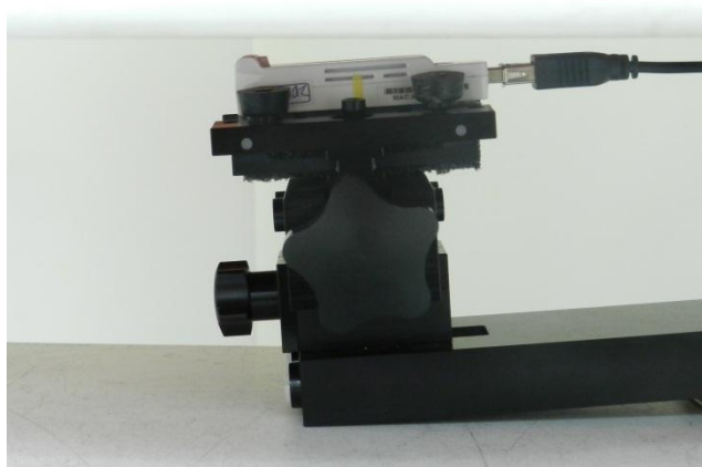
Horizontal Down with Phantom 5 mm Gap Antenna swivel 0 degree
