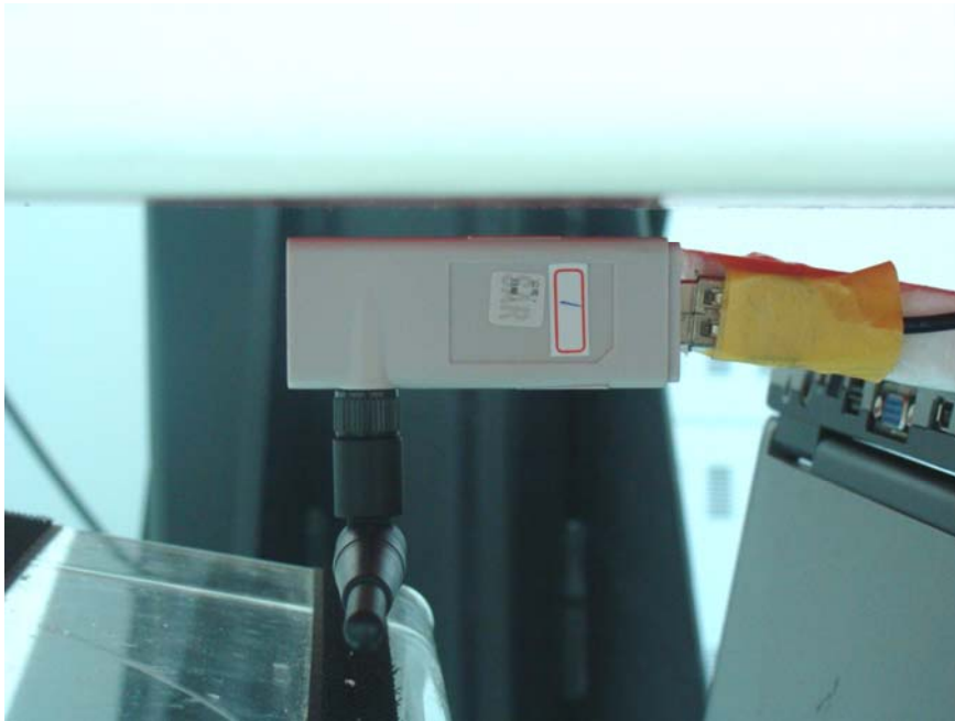
USB Configuration 2 and Antenna set Perpendicular
