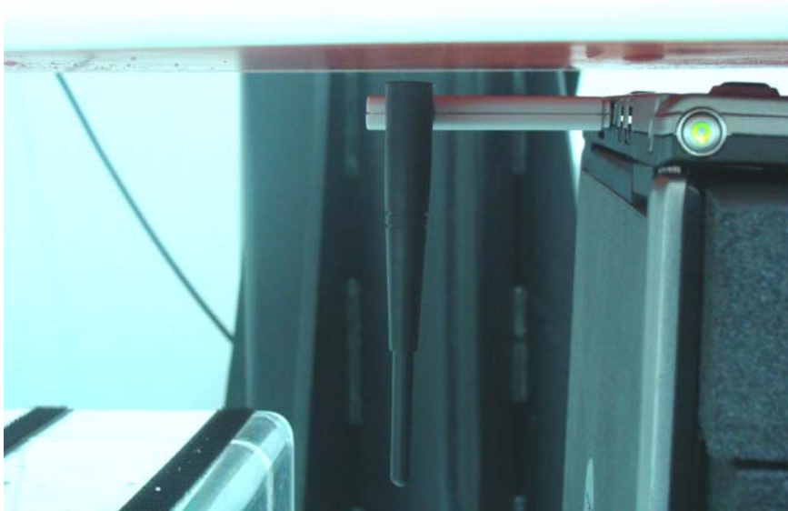
USB Configuration 1 and Antenna set Perpendicular
