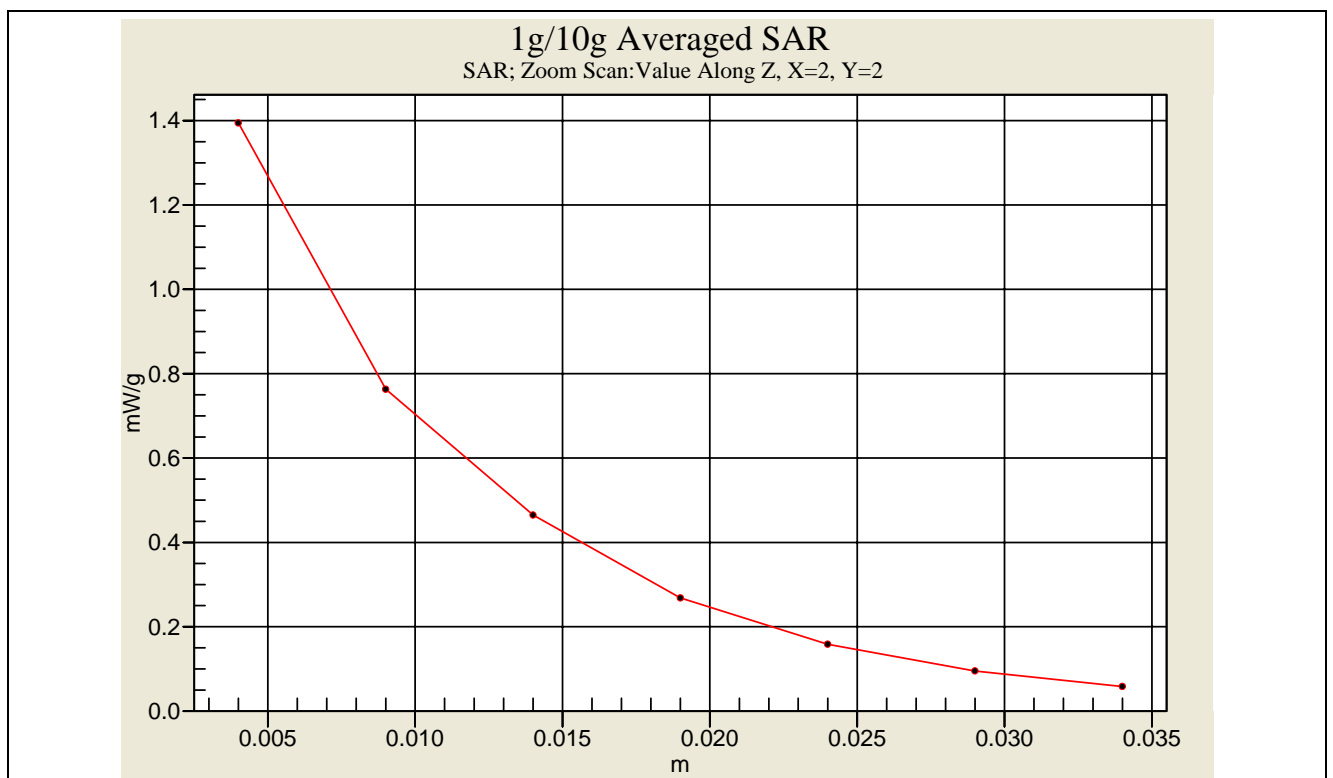
SAR Measurement _ Flat 802.11g CH6(Bottom)
