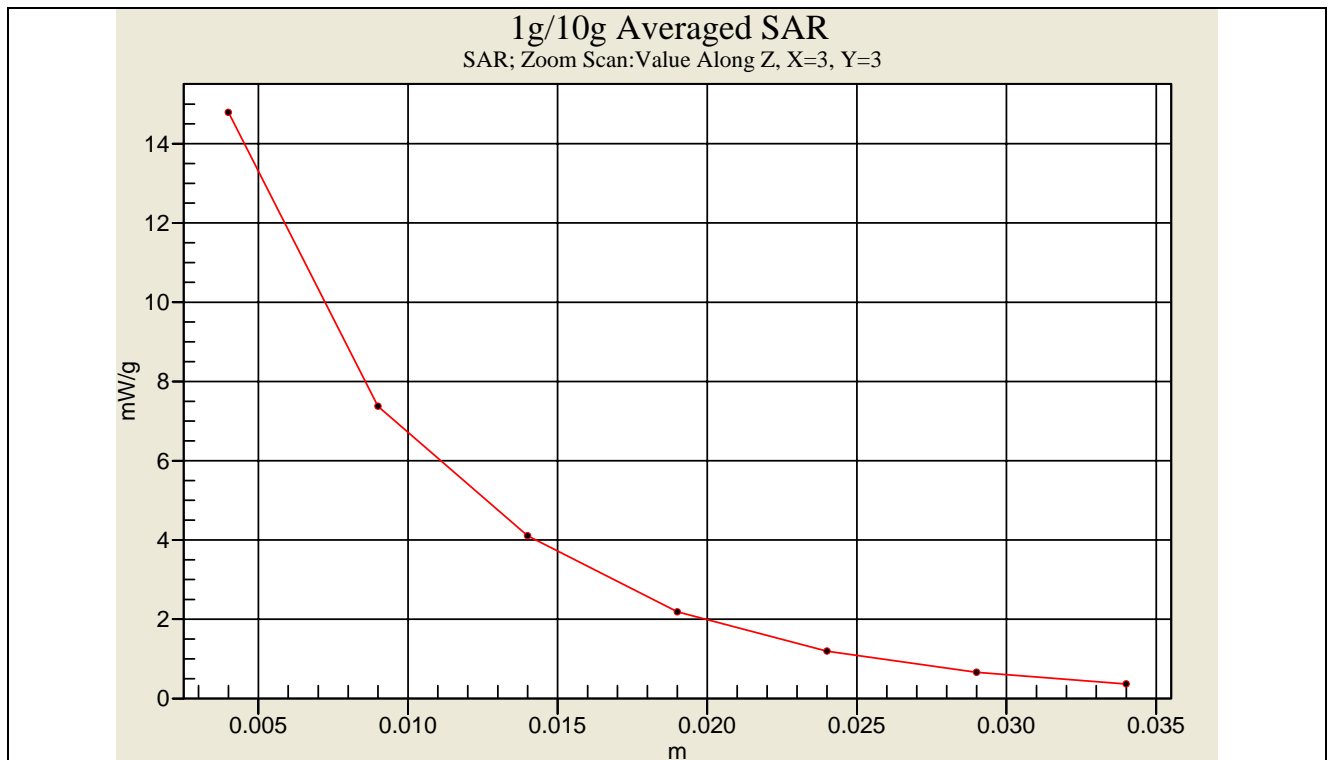
Head-Tissue-Simulating-Liquid 2GHz(20070508)
