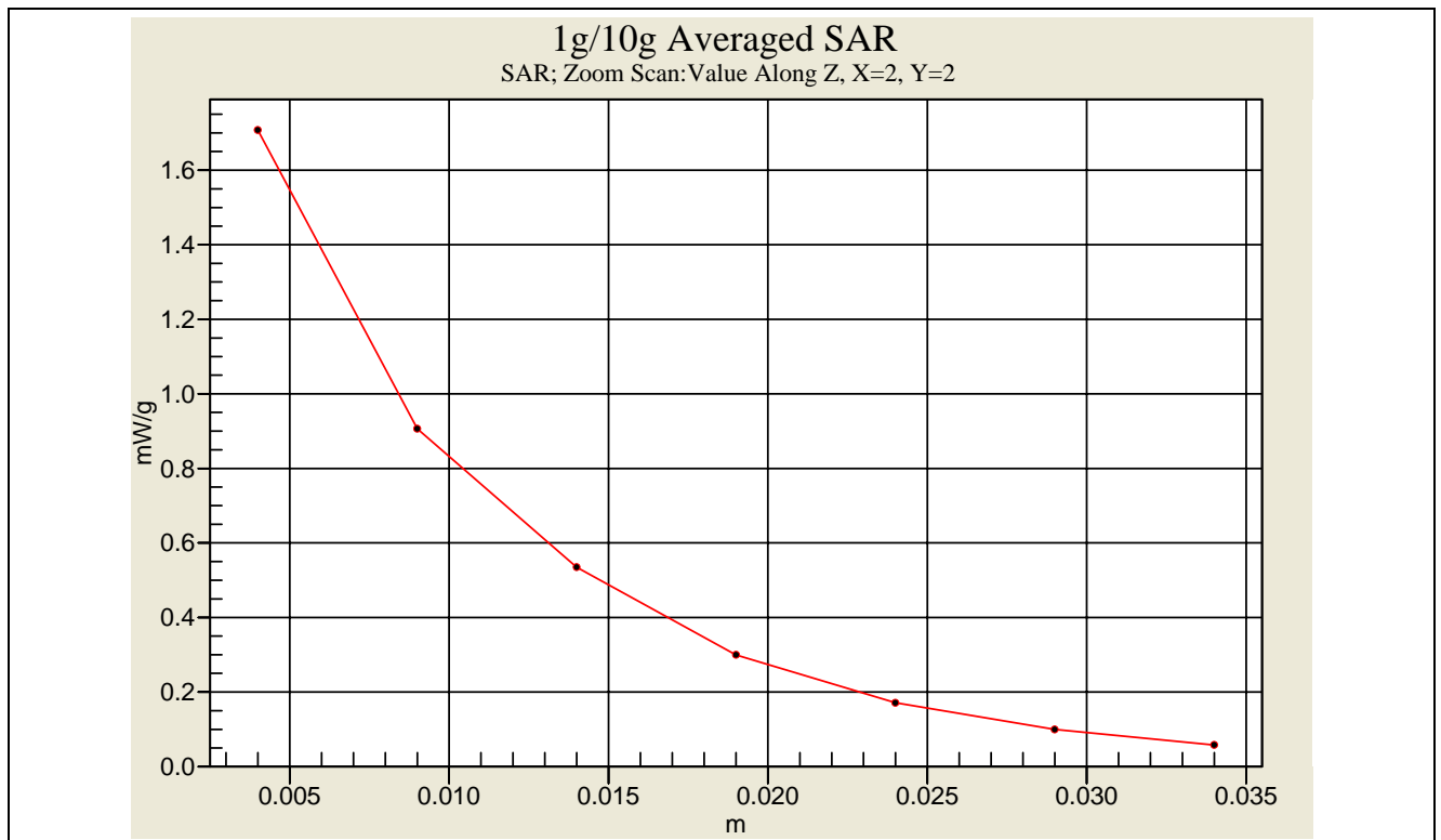
SAR Measurement _ Flat 802.11n_40MHz CH6(Buttom)
