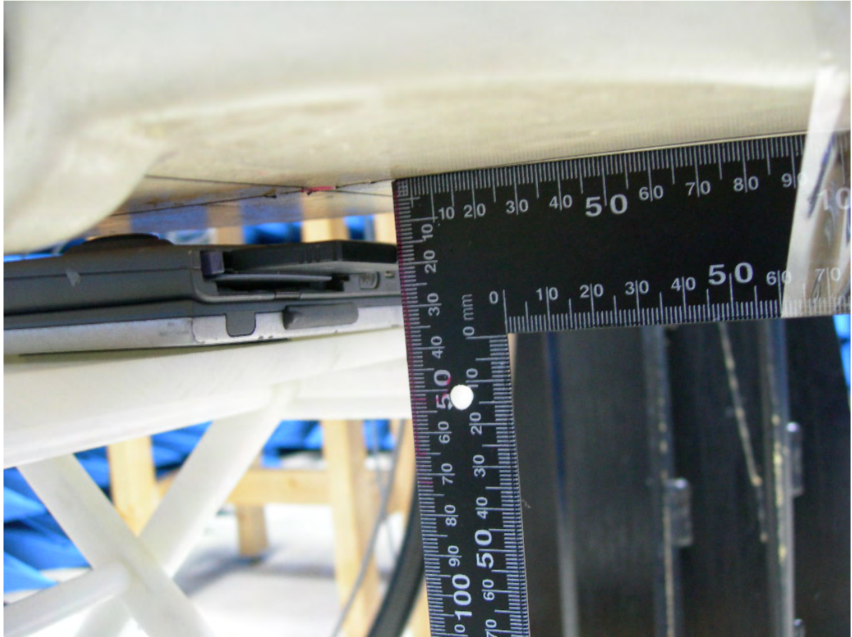
Figure 12.Body SAR Test Setup (Flat Section)_Bottom
