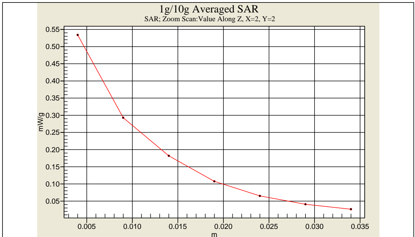
SAR Measurement _ Flat Cheek 802.11b CH11(Tip)
