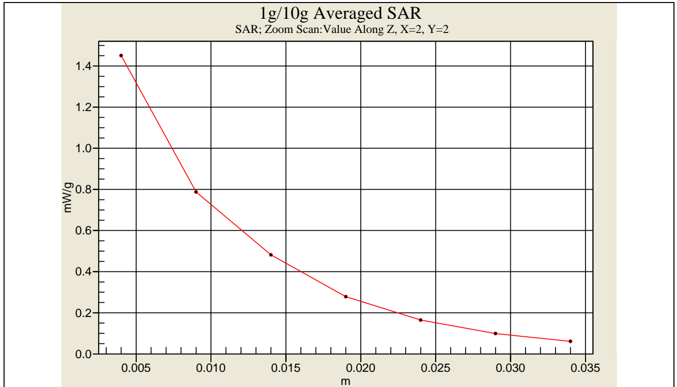
SAR Measurement _ Flat 802.11n_20MHz CH1(Buttom)
