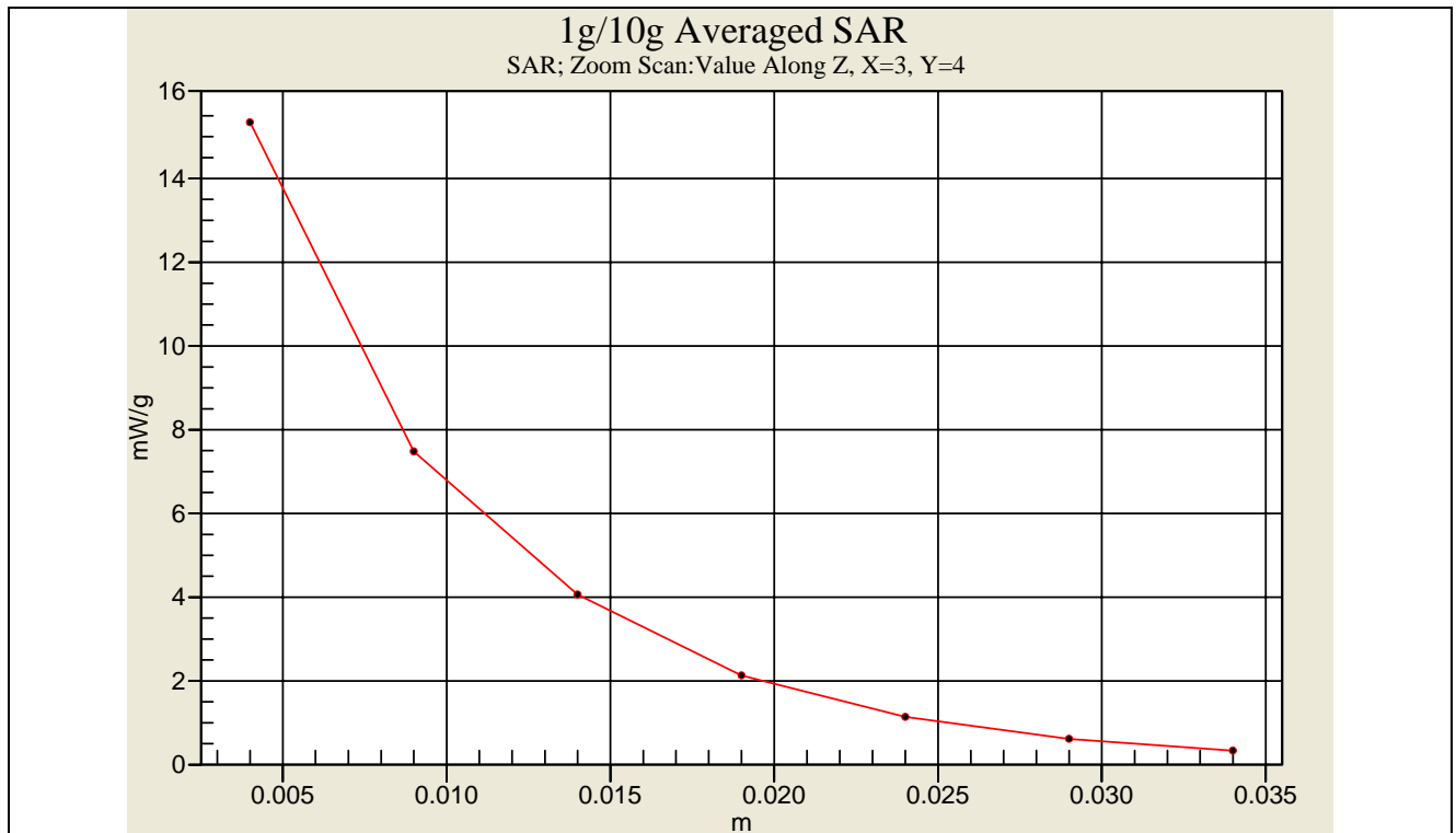
Head-Tissue-Simulating-Liquid 2GHz(20070421)
