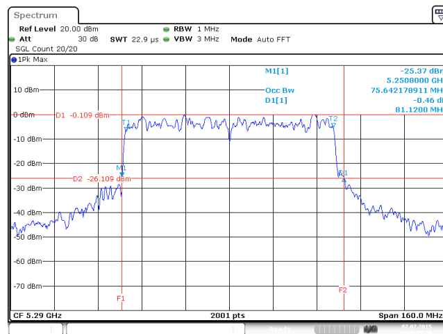
5250-5350MHz - Worst Emission 26Bandwidth Plots
