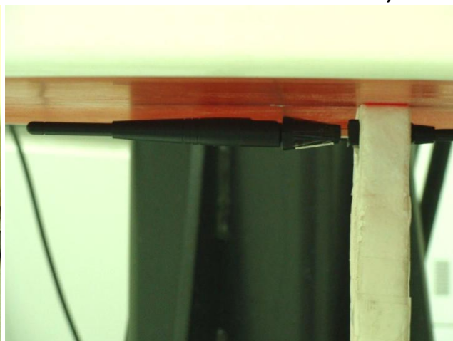
USB Configuration 2 (Horizontal Down with Phantom 0.5 cm Gap and Antenna set Straight)
