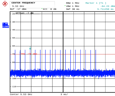
Radar #0 DFS detection threshold level
