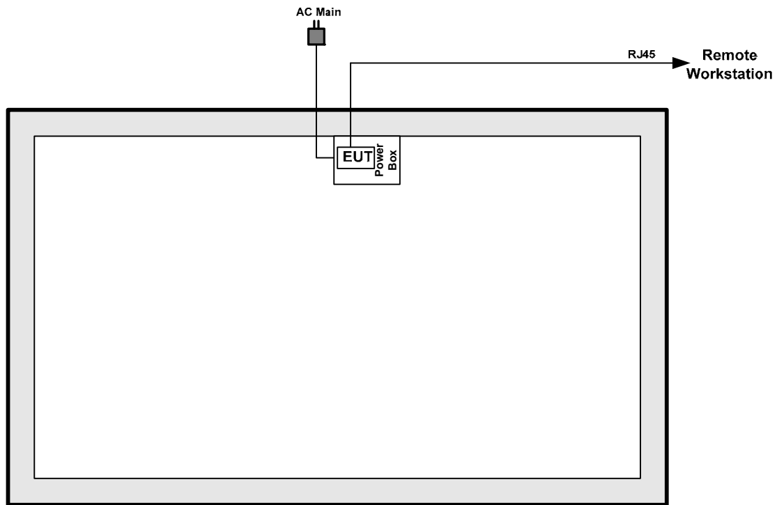
Test Setup Diagram - Radiated Test (Above 1GHz)
