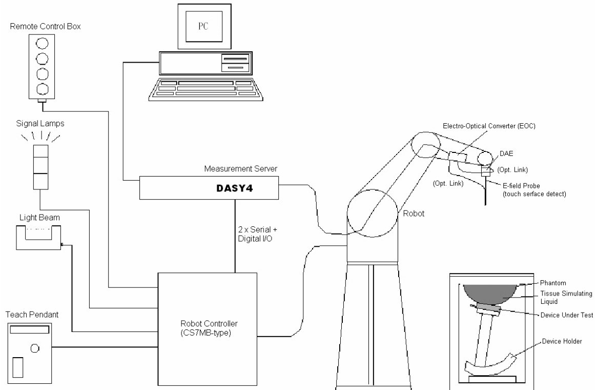
Fig. 4.1 DASY4 system
