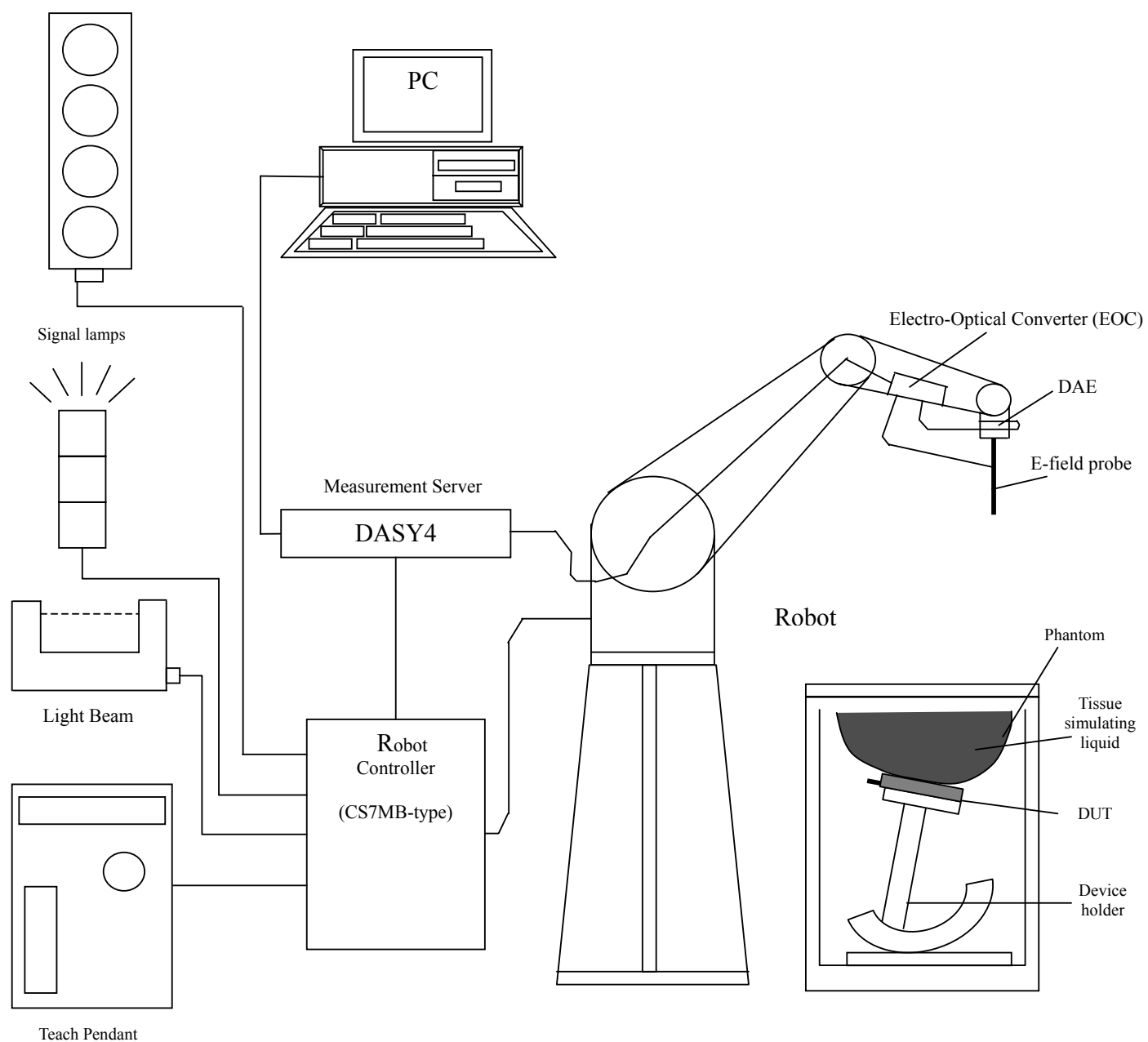
Fig. 5.1 DASY4 system
