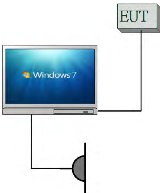
Fig. 2-2 AC Power Line Conducted Emission
