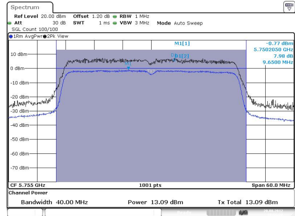
11N5.8G-40M – F4 [Port 2]
