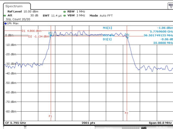
11N5.8G-40M – F5 [Port 2]
