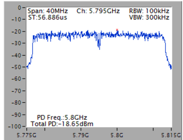
11N5.8G-40M – F5 [Sum All Chains]
