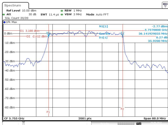
11N5.8G-40M – F4 [Port 1]
