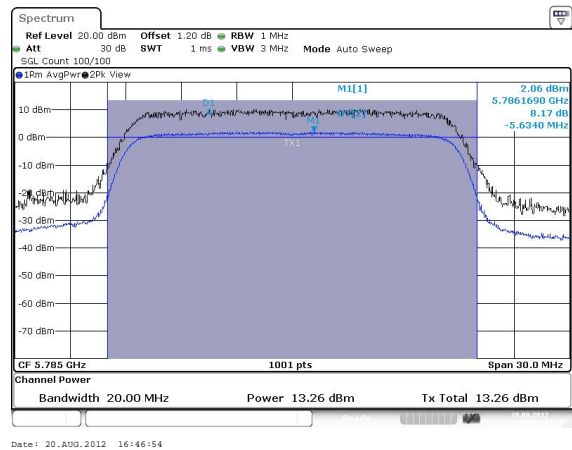
11N5.8G-20M – F3 [Port 2]
