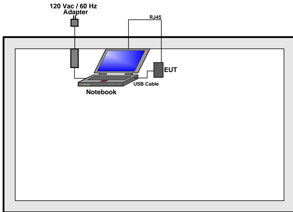
Test Setup Diagram - Radiated Emission Test (Above 1GHz)
