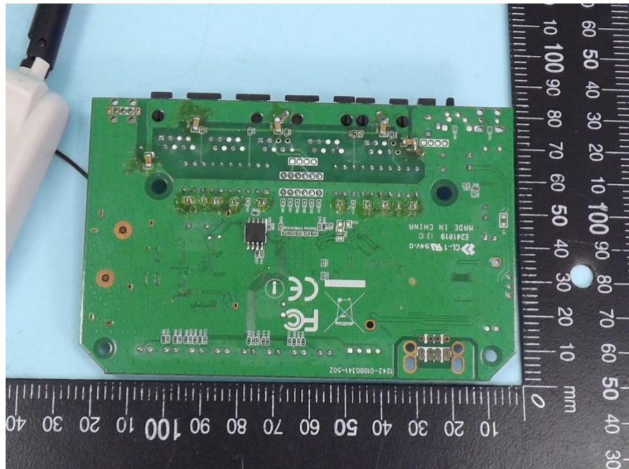
Sample 2 with Ant. No. 4 (Part No. RFA02-5C15S0-70B55W1)
