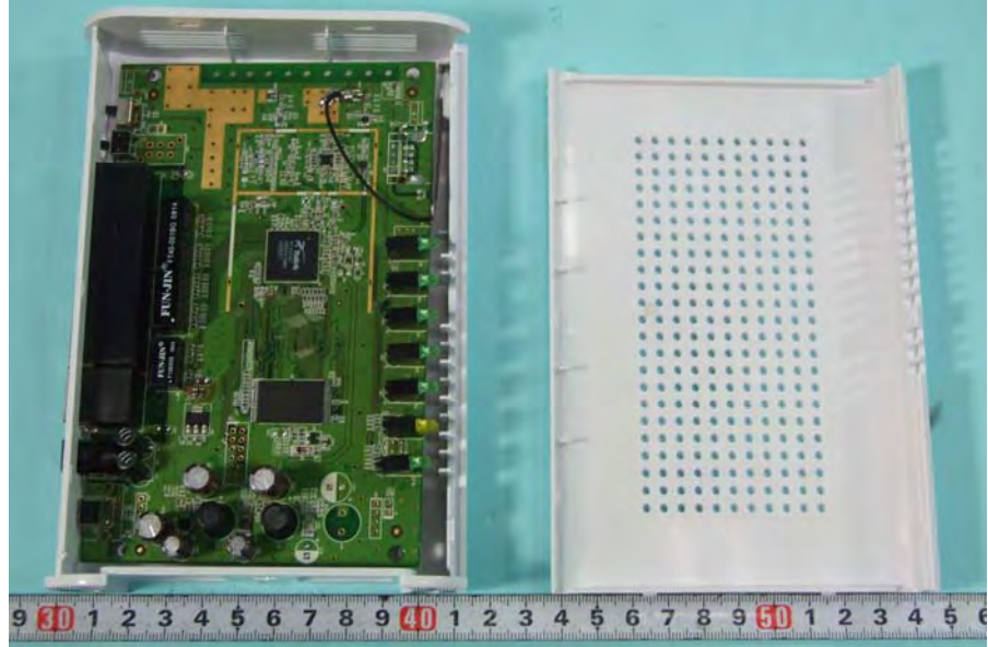
PIFA antenna without USB port
