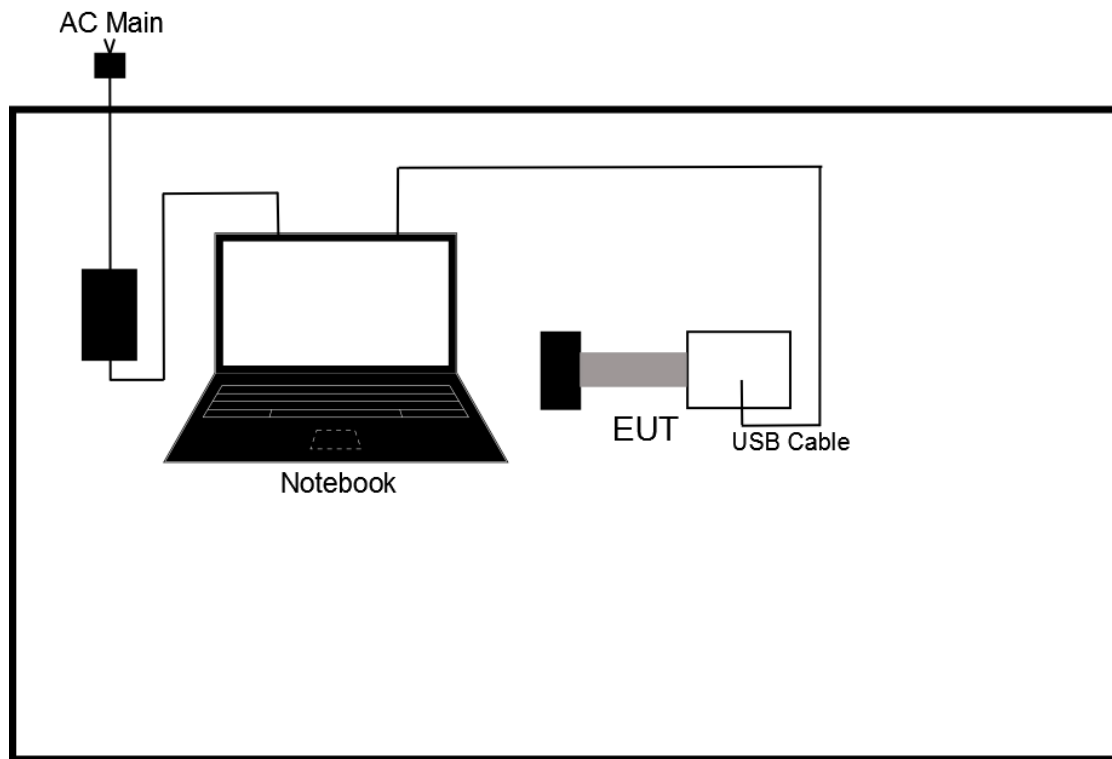
Test Setup Diagram - Radiated Test_ Above 1GHz
