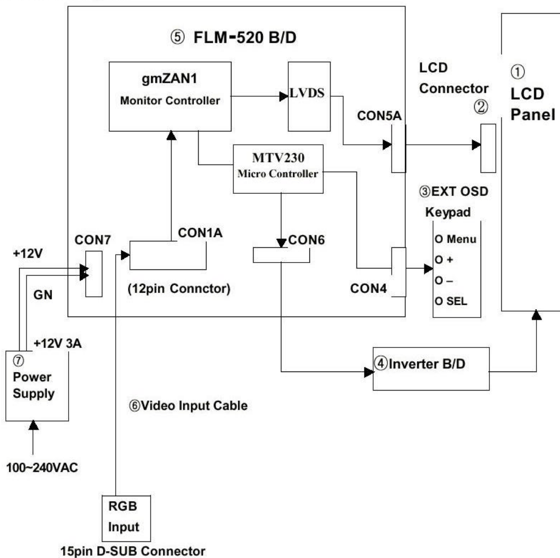
FLM-520 Block Diagram
