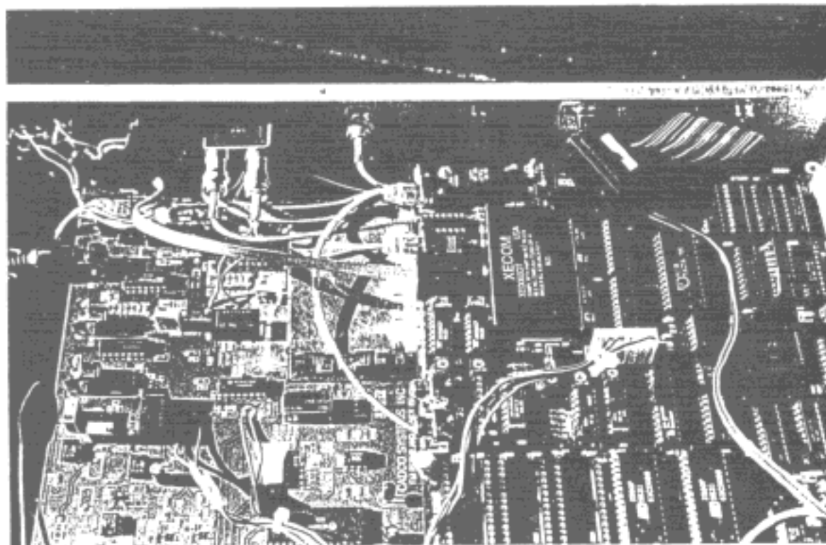
Photo 4: INTERIOR VIEW SHOWING ADDED FERRITE BEAD ON RS232 CONNECTOR
