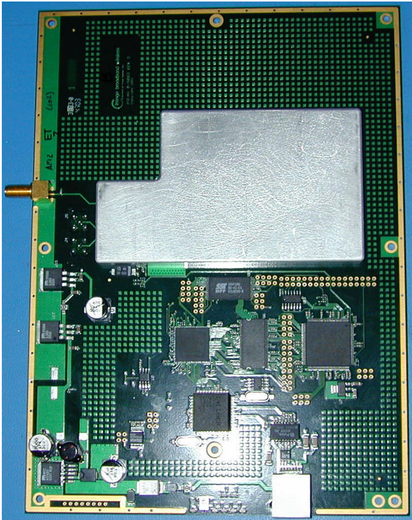
NCYM900S Pictures – Internal with shield on
