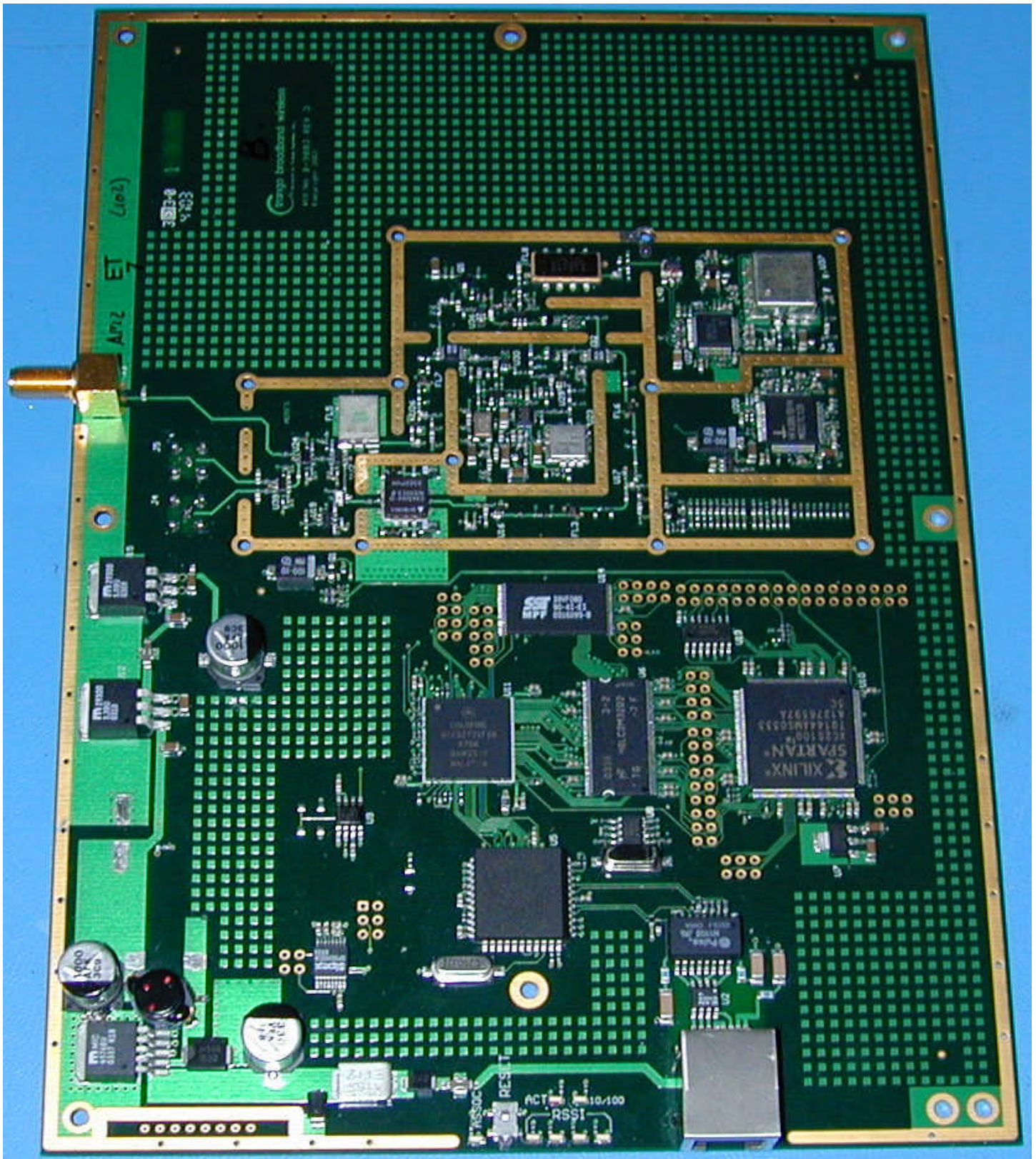
NCYM900S Pictures – Internal with shield off
