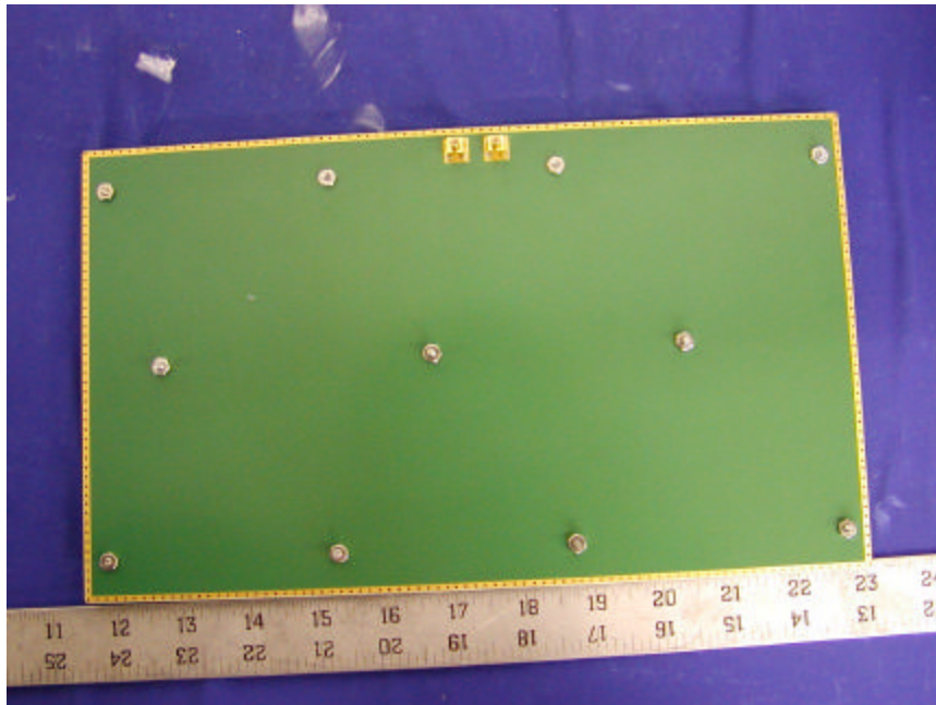
EUT – Antenna Solder View
