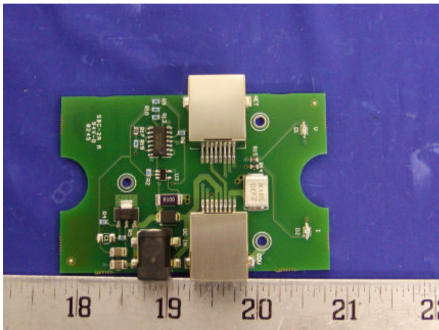
Adapter Component View
