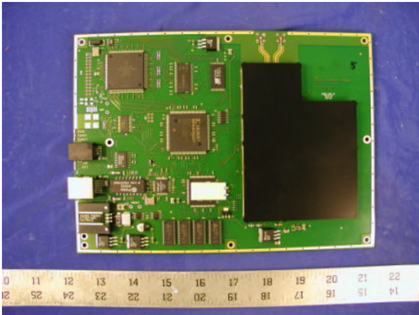
EUT – Component View with Sub Shield
