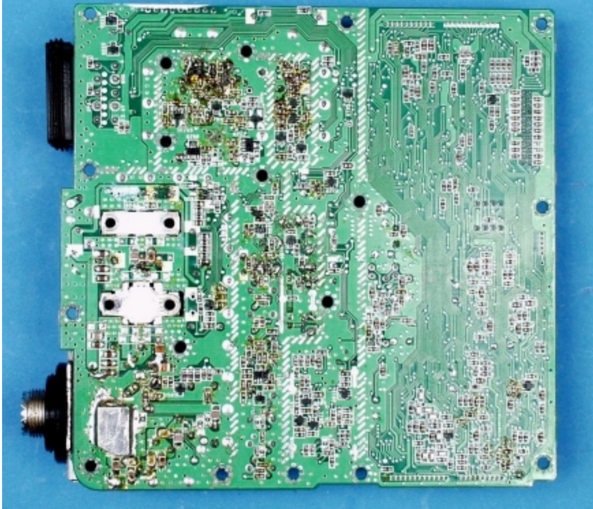
Midland 511C Circuit Board Track Side
