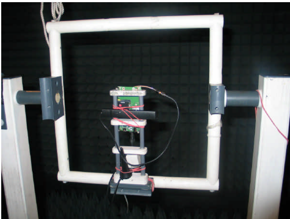
Photo 6: Setup for radiated tests (EUT B operated in a cradle and with external antenna)
