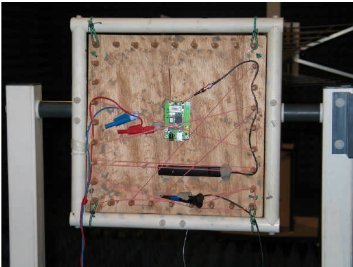
Photo 5: Setup for radiated tests (EUT A operated in a cradle and with external antenna)
