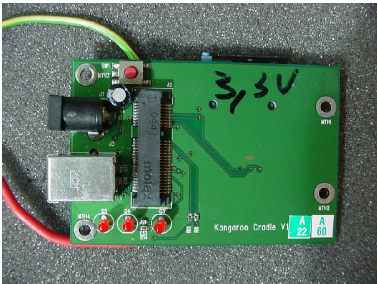
Photo 7: Cradle AE1 (front side)
