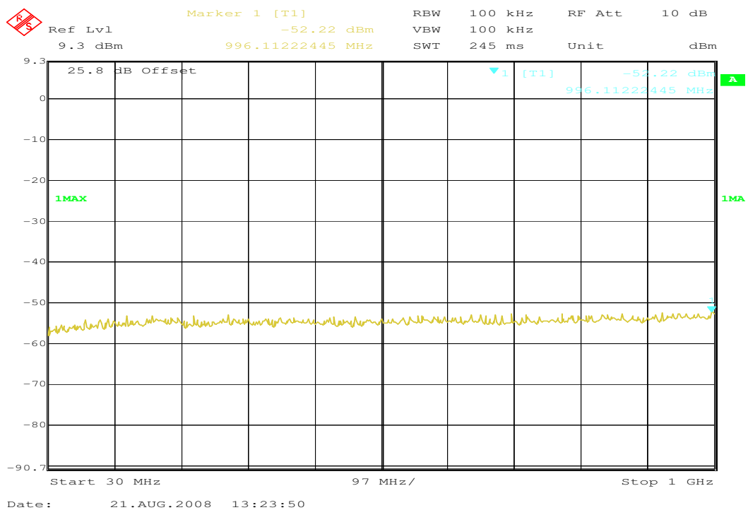
Plot 13: 30 MHz – 1 GHz (Middle Channel)
