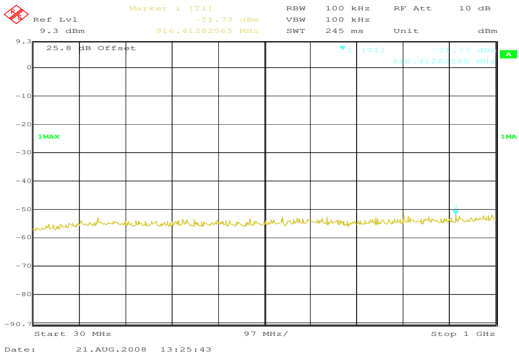
Plot 16: 30 MHz – 1 GHz (Highest Channel)
