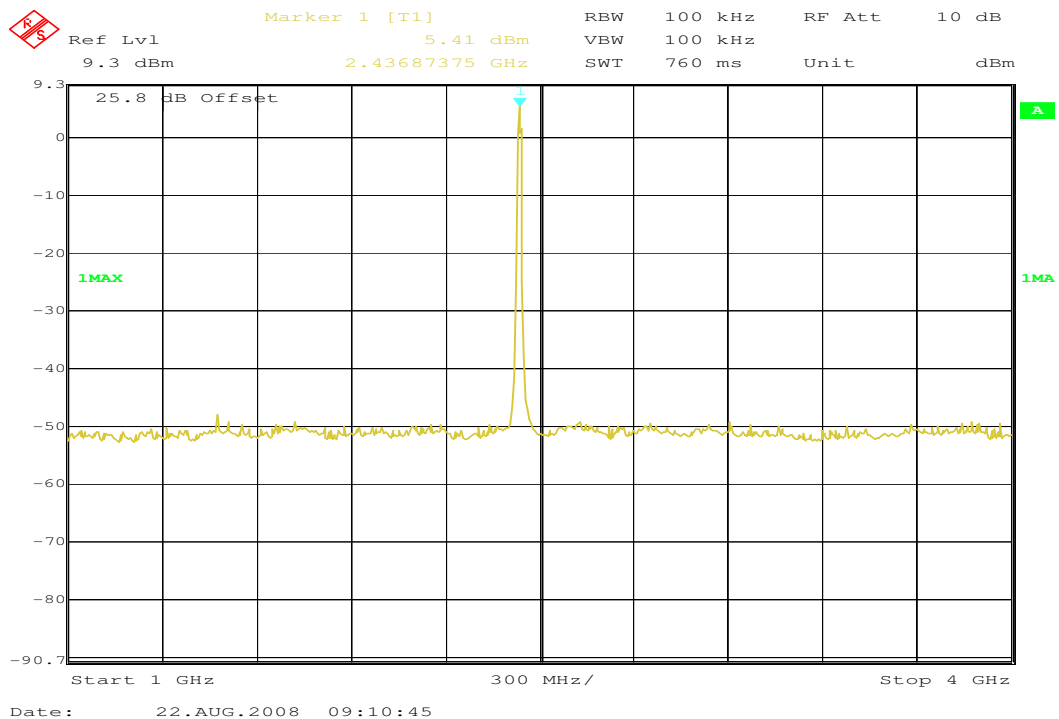
Plot 14: 1 GHz – 4 GHz (Middle Channel)
