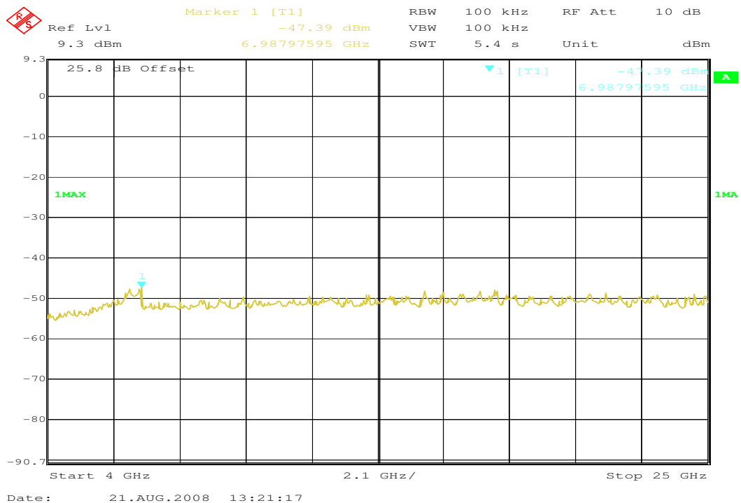
Plot 12: 4 GHz – 25 GHz (Lowest Channel)
