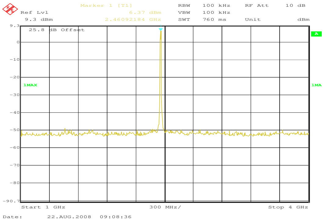
Plot 17: 1 GHz – 4 GHz (Highest Channel)
