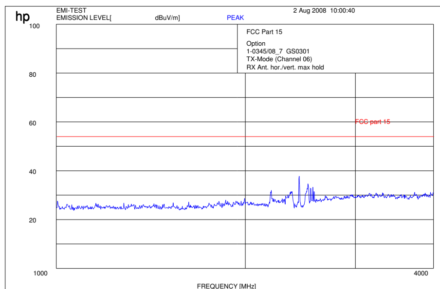
Plot 16: 1 - 4 GHz (middle channel)
