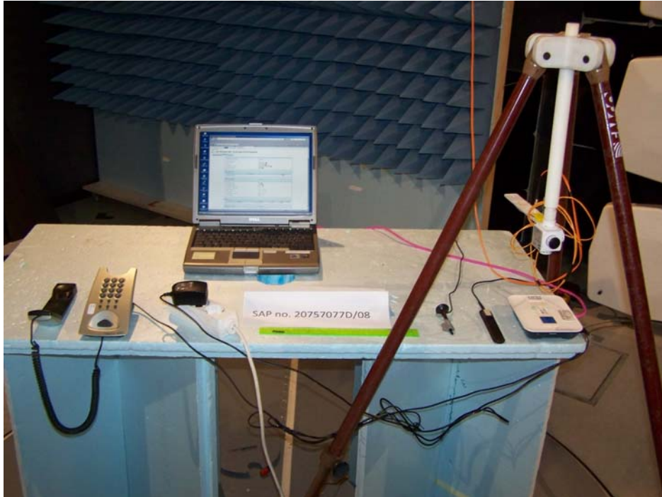
Photograph 5: Test Set-up
