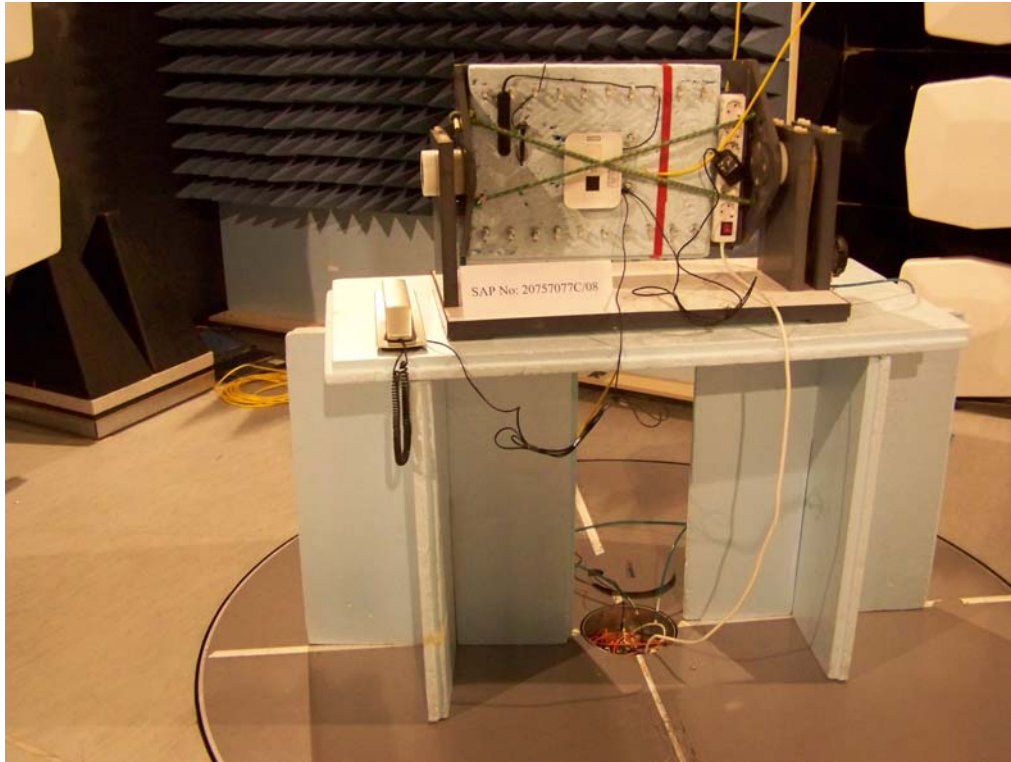
Photograph 3: Radiated field strength measurements, set-up 3
