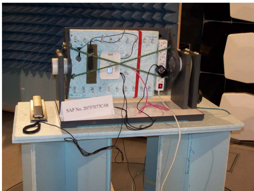
Photograph 2: Radiated field strength measurements, set-up 1
