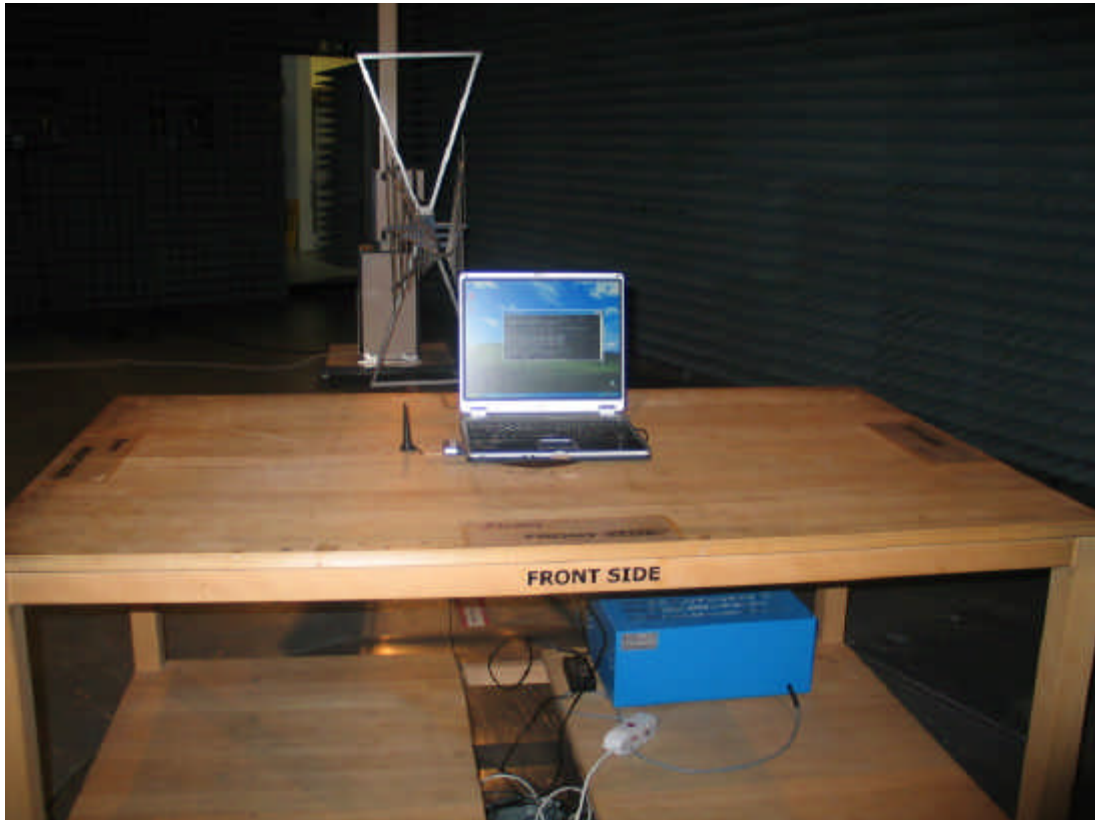
Picture 2: Setup for radiated measurements below 1 GHz
