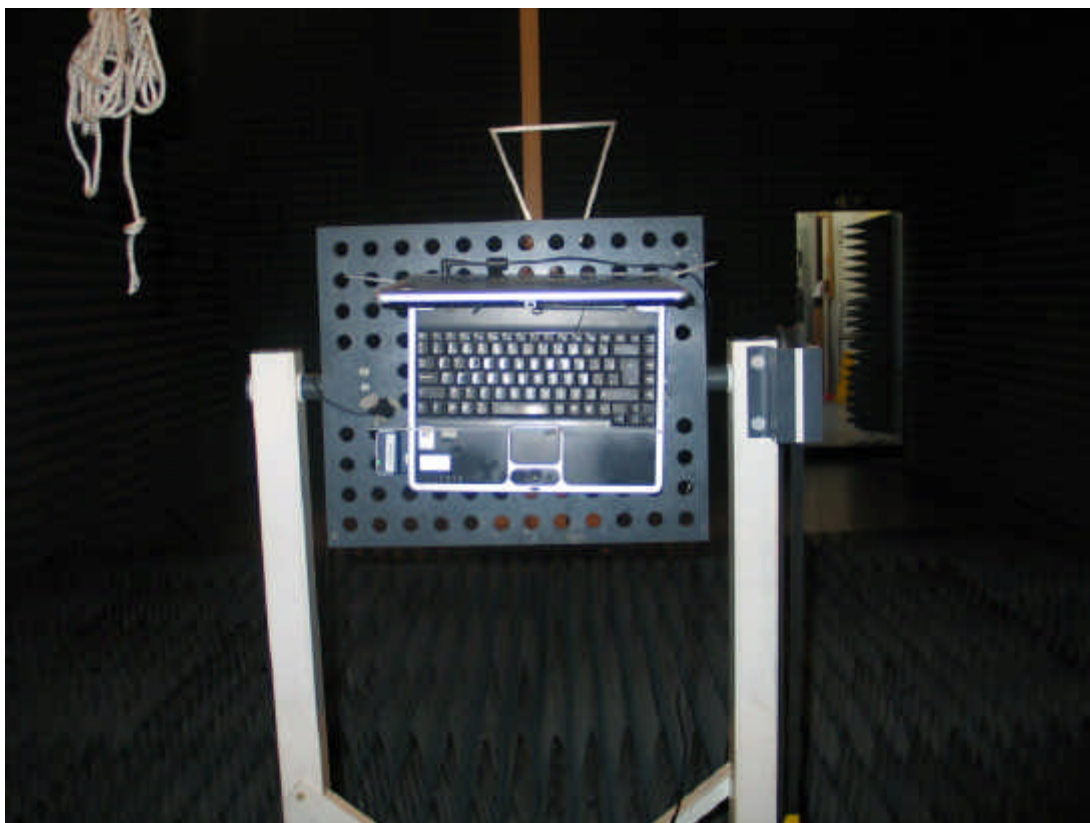
Picture 3: Setup for radiated measurements above 1 GHz
