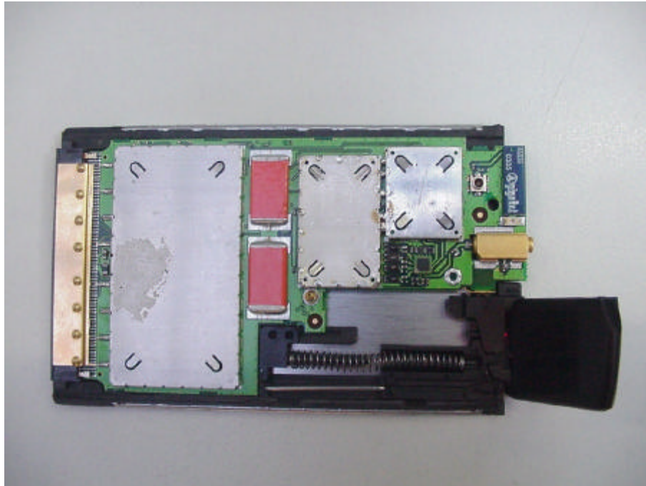
Picture 1 : EUT (top side, without housing)
