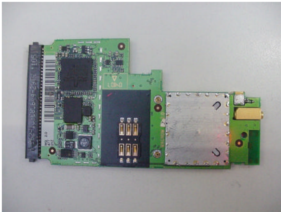
Picture 2 : EUT (bottom side, without housing)
