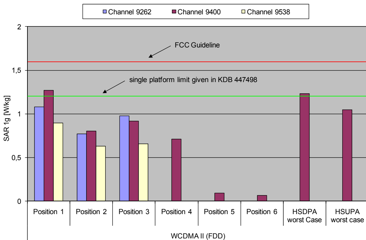
Fig. 9: The measured SAR values for the Option XYfi for WCDMA II (FDD) in comparison to the FCC exposure limit.
