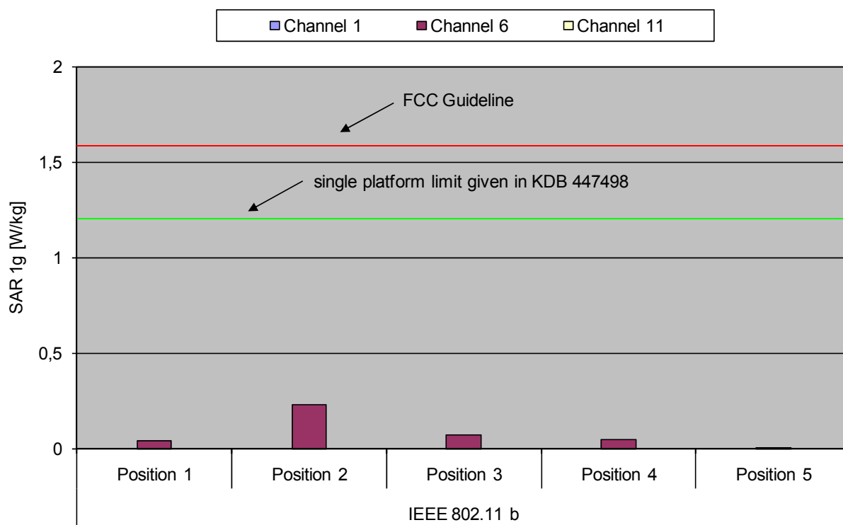
Fig. 10: The measured SAR values for the Option XYfi for IEEE 802.11 b in comparison to the FCC exposure limit.
