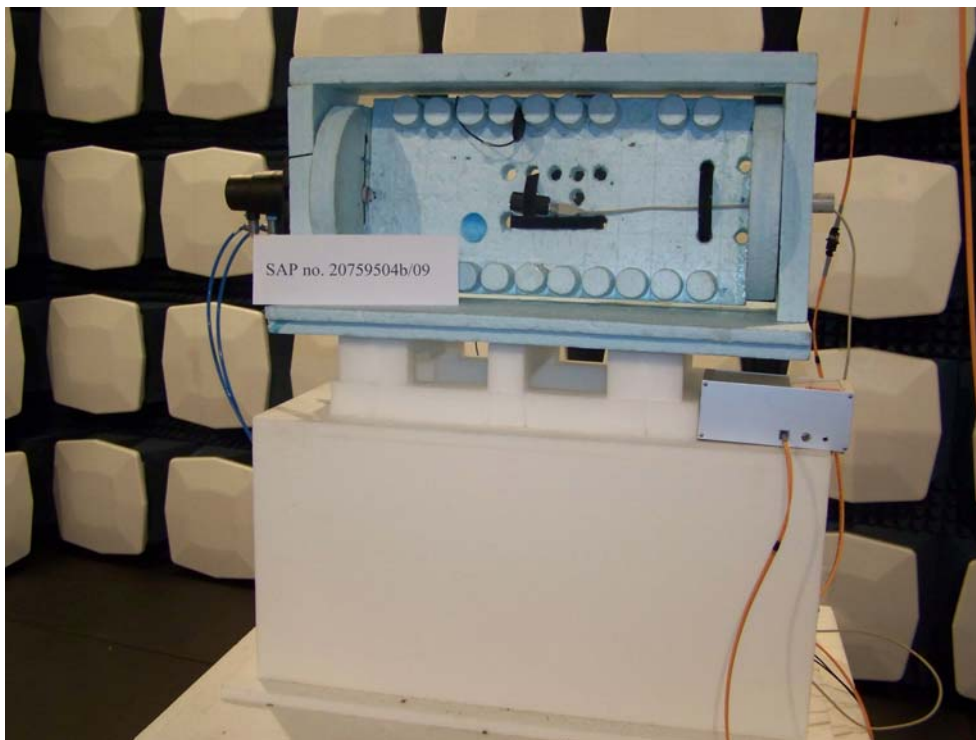
Photograph 2: Equipment under test: Radiated set-up
