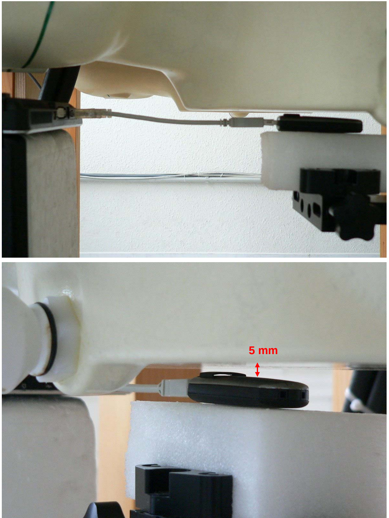
Fig. 21: Position B with the Fujitsu Siemens Amilo Pro.
