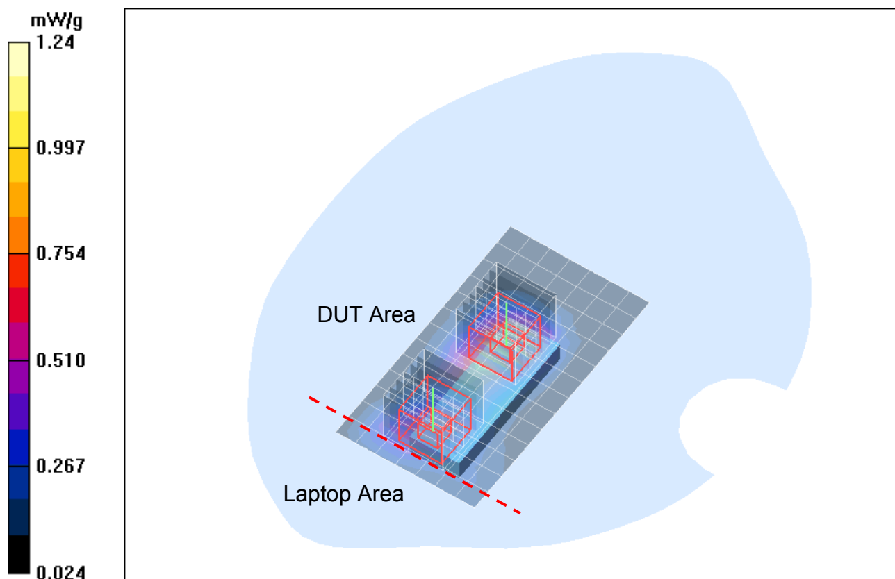
Fig. 13: SAR distribution for GPRS 1900 (Class 10), channel 810, Position A (Fujitsu Siemens Amilo Pro, September 29, 2009; Ambient Temperature: 21.3^{\circ}\text{C} ; Liquid Temperature: 20.8^{\circ}\text{C} ).
