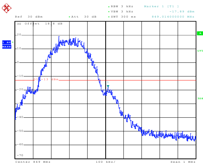
Higher Band Edge Plot on Channel 251
