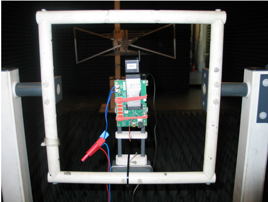
Photo 3: Setup for radiated tests
