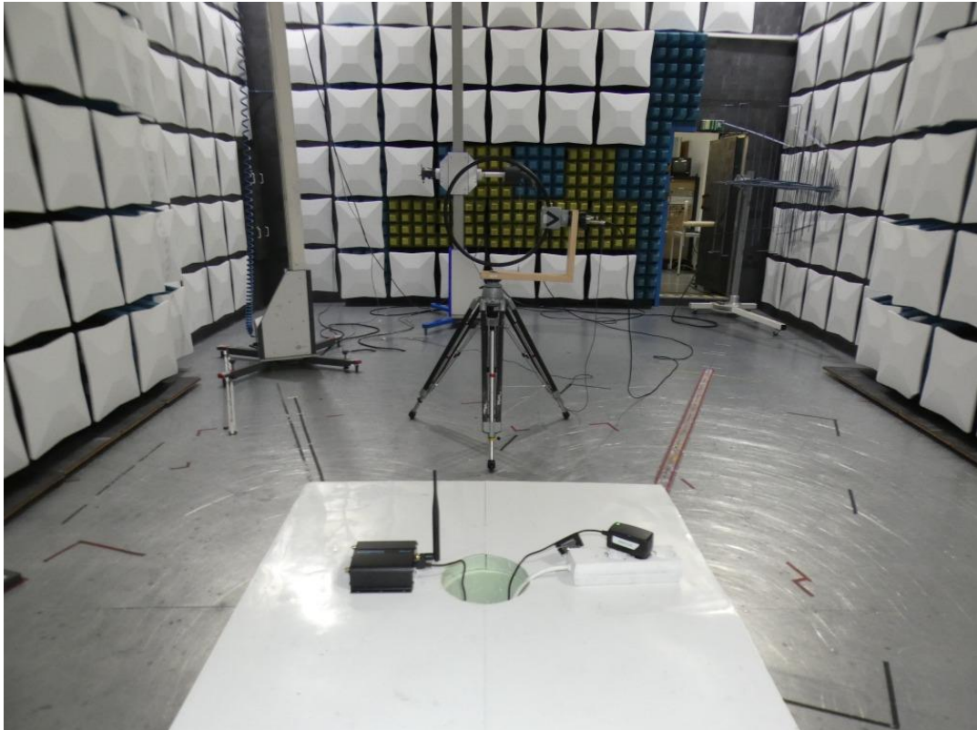
Photo 1: Test setup for radiated measurements below 30 MHz (H-Field, SAC)
