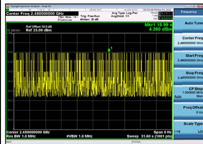
DQPSK,2480,2DH5,Transmission Number
