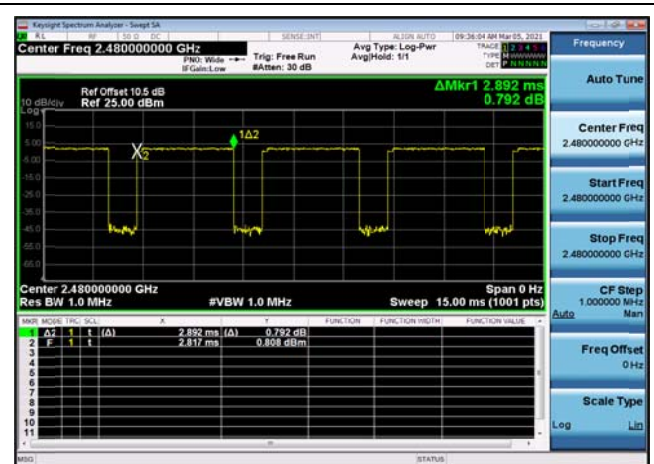
8DPSK,2480,3DH5,Transmission Time
