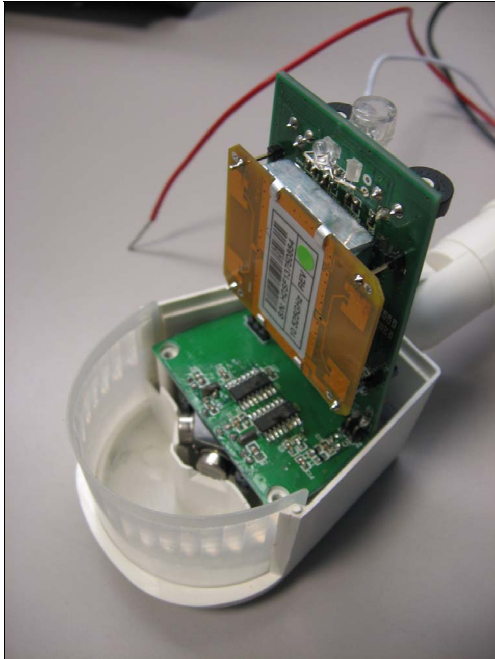
Figure 1: Internal Photos - Assembled
