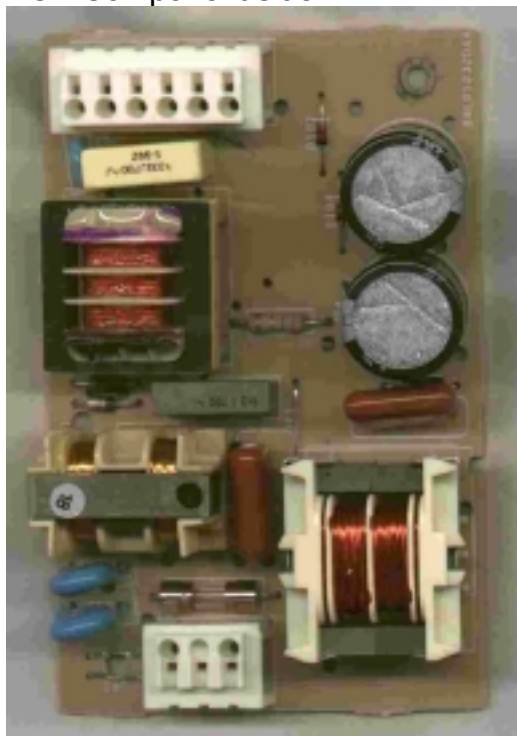
PCB Component side
