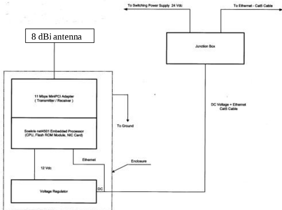
Figure 1. Block Diagram of Wireless Outdoor Mount Ethernet NCB5L9102A Bridge
