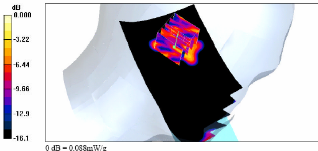
Head-SAR Test Result for Left Tilted Position – Channel 1
