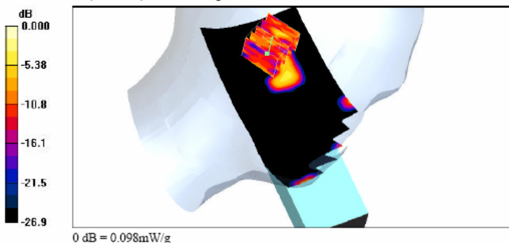
Head-SAR Test Result for Left Tilted Position – Channel 70
