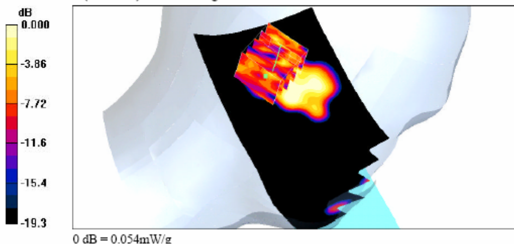
Head-SAR Test Result for Left Cheek Position – Channel 70
