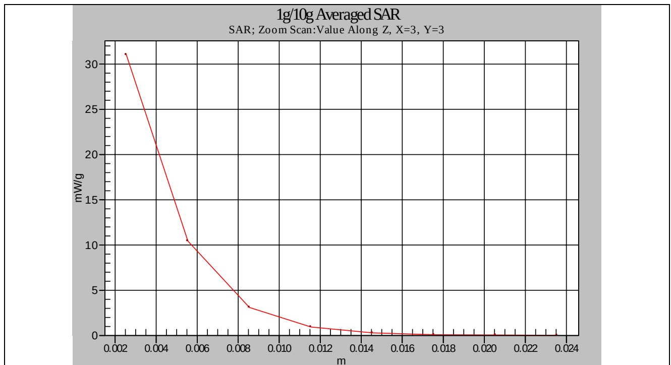
Body-Tissue-Simulating-Liquid 5.8GHz
