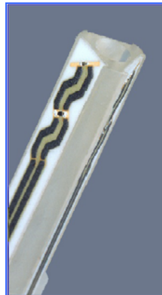
Figure 8. EX3DV3 E-field Probe
