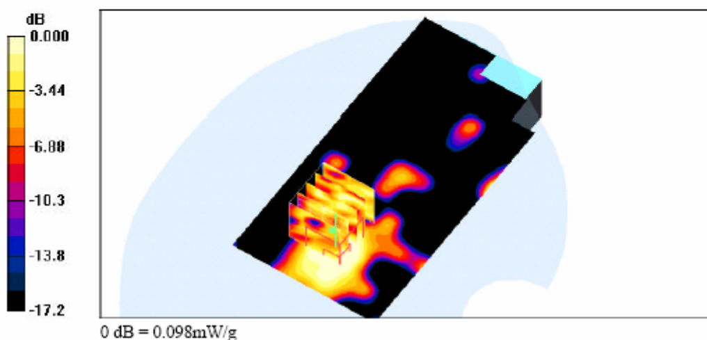
Body-SAR Test Result for Flat Position – Channel 70
