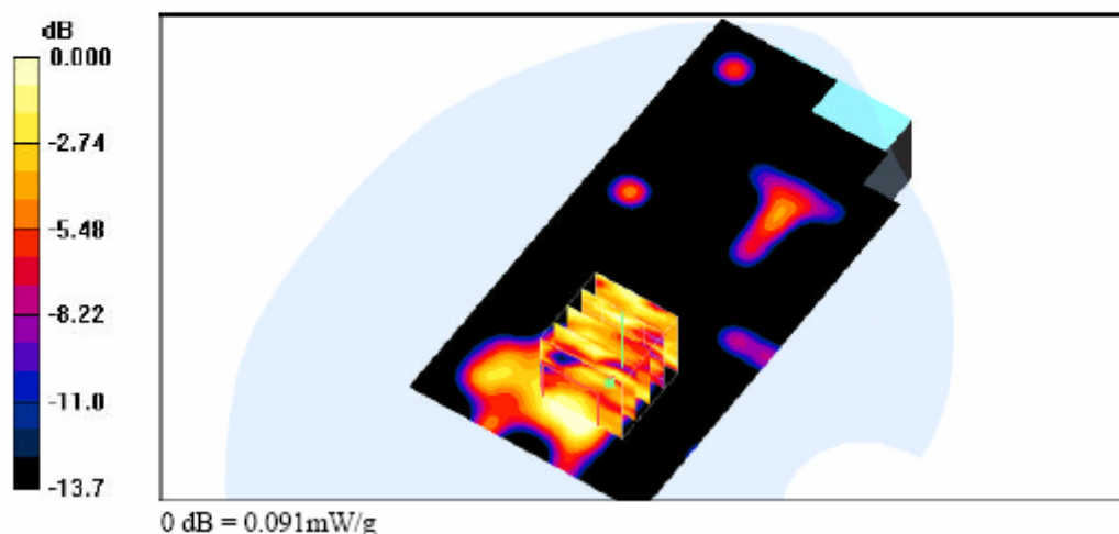
Body-SAR Test Result for Flat Position – Channel 1
