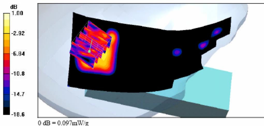
Head-SAR Test Result for Right Tilted Position – Channel 70
