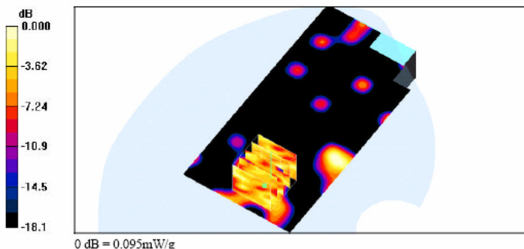
Body-SAR Test Result for Flat Position – Channel 139
