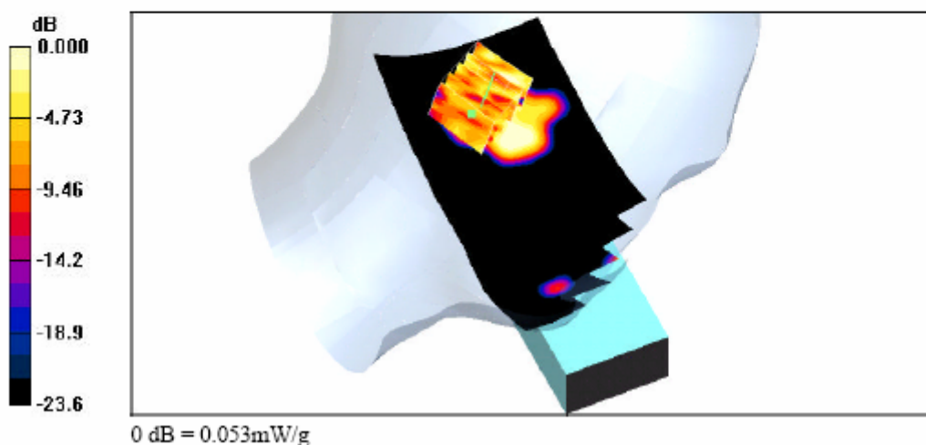
Head-SAR Test Result for Left Cheek Position – Channel 139
