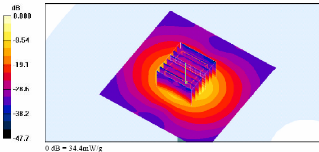
Head-Tissue-Simulating-Liquid 5.8GHz
