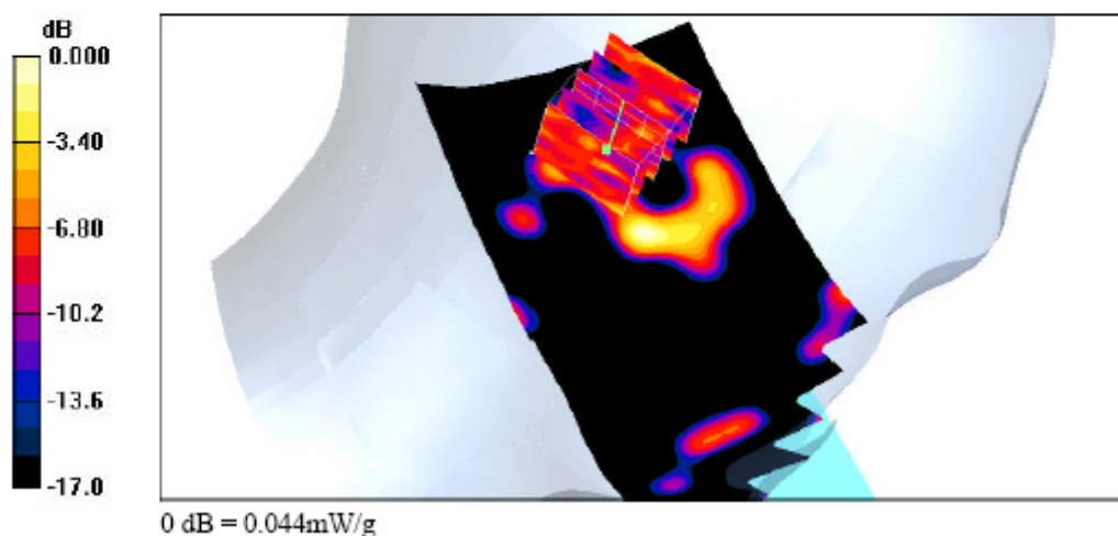
Head-SAR Test Result for Left Cheek Position – Channel 1
