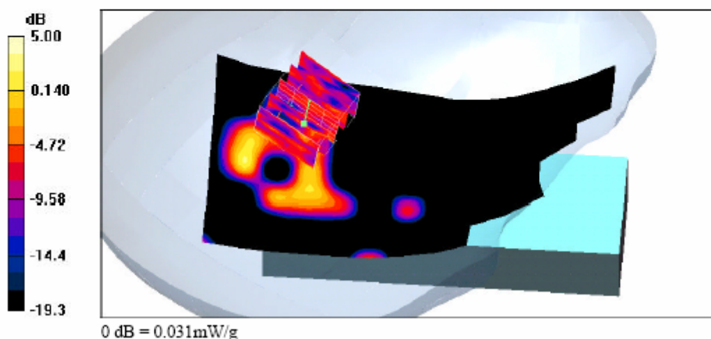
Head-SAR Test Result for Right Cheek Position – Channel 139
