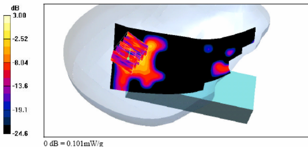
Head-SAR Test Result for Right Tilted Position – Channel 139
