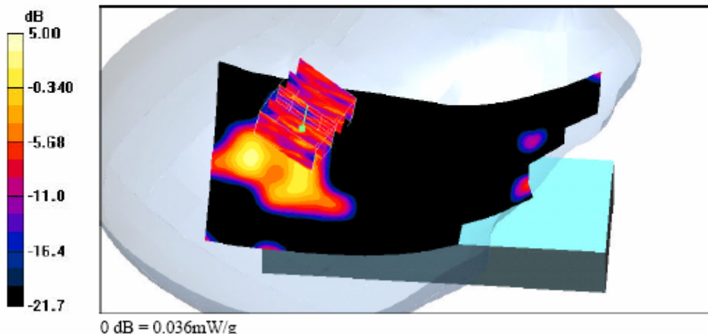
Head-SAR Test Result for Right Cheek Position – Channel 70
