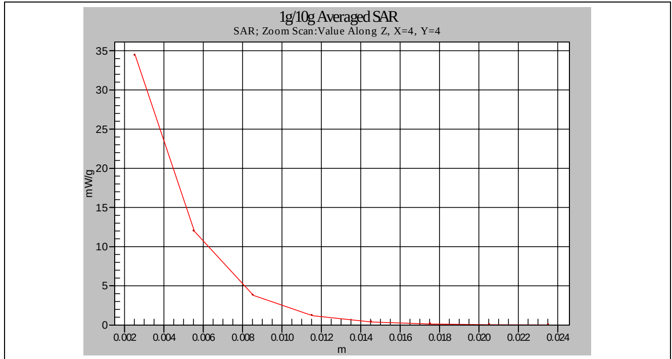
Head-Tissue-Simulating-Liquid 5.8GHz
