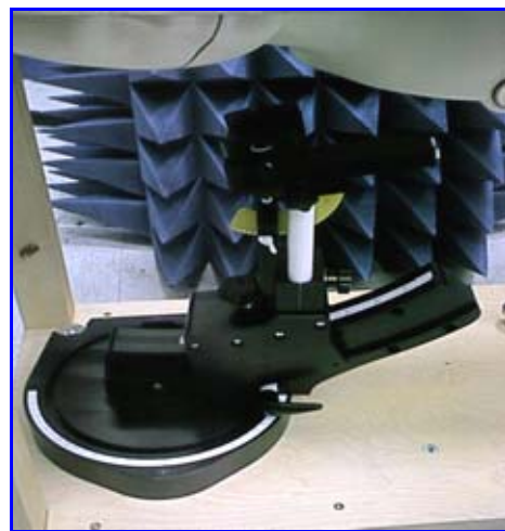
Figure 10. Device Holder
