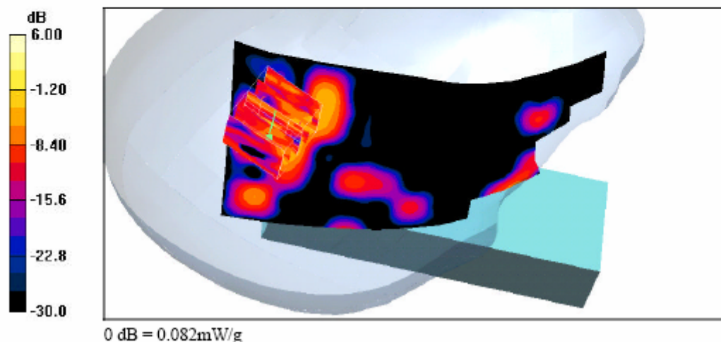
Head-SAR Test Result for Right Tilted Position – Channel 1
