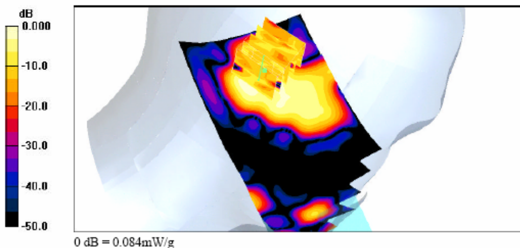
Head-SAR Test Result for Left Tilted Position – Channel 139
