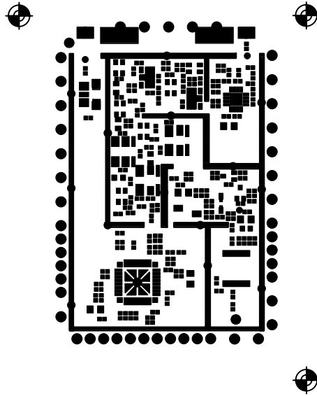
COMP. MASK
